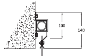
Outside Opening
